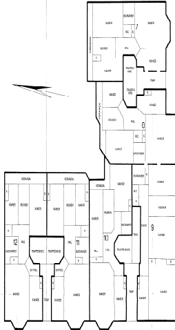
1 e VERDEPING 1:100
